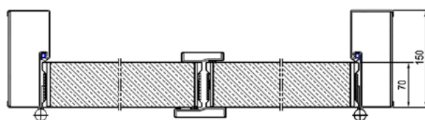
Double-leaf door HC 90XL - 2
