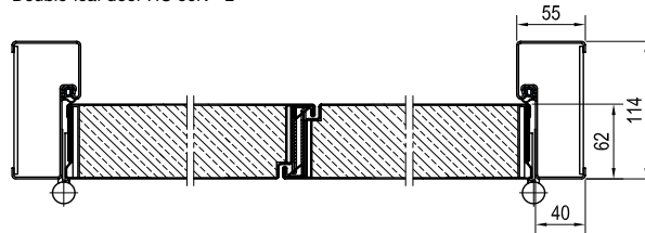
Double-leaf door HC 60N - 2
